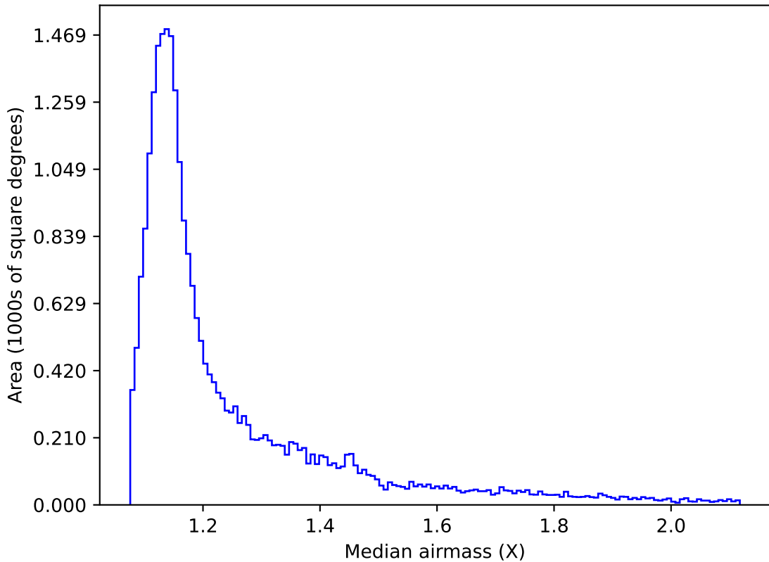
ddf_acor_sf10_lsf30_lsr20_v3.4_10yrs All sky g band: Median airmass
