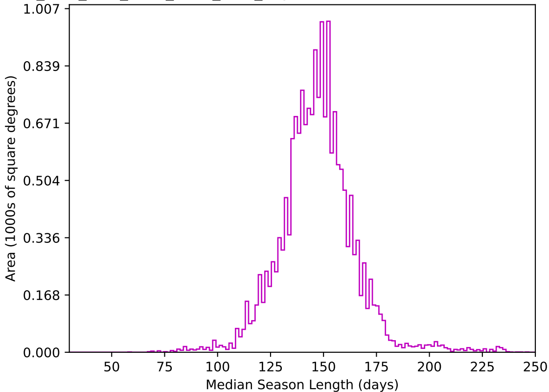
ddf_acor_sf10_lsf30_lsr20_v3.4_10yrs WFD z band: Median Season Length
