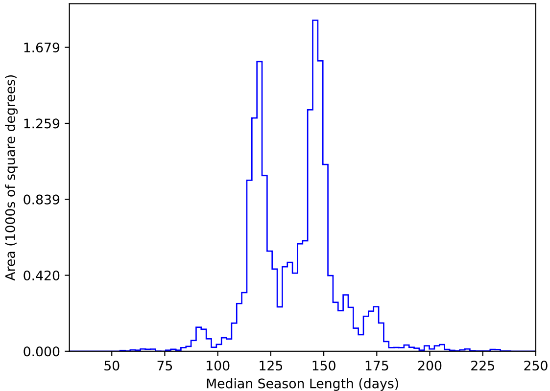
ddf_acor_sf10_ls30_lsr20_v3.4_10yrs WFD y band: Median Season Length
