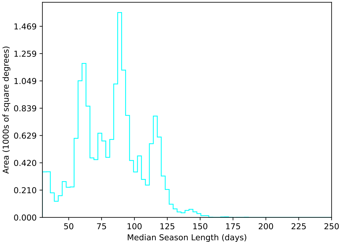
ddf_acor_sf10_lsf30_lsr20_v3.4_10yrs WFD u band: Median Season Length
