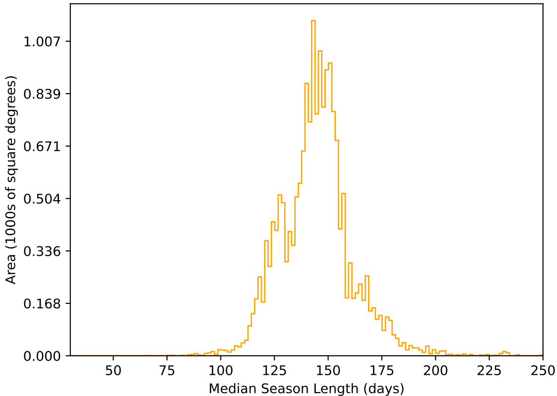
ddf_acor_sf10_lsf30_lsr20_v3.4_10yrs WFD r band: Median Season Length
