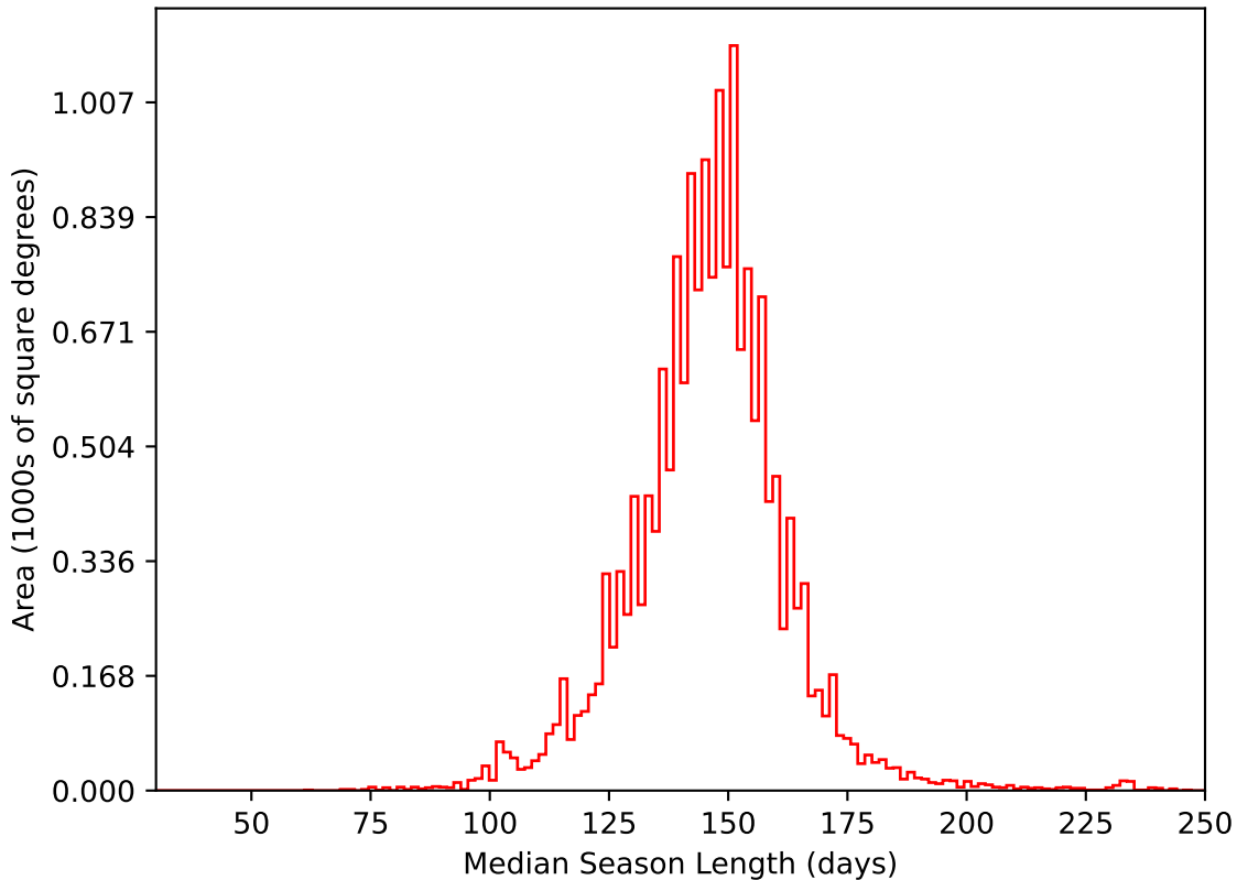
ddf_acor_sf10_lsf30_lsr20_v3.4_10yrs WFD i band: Median Season Length
