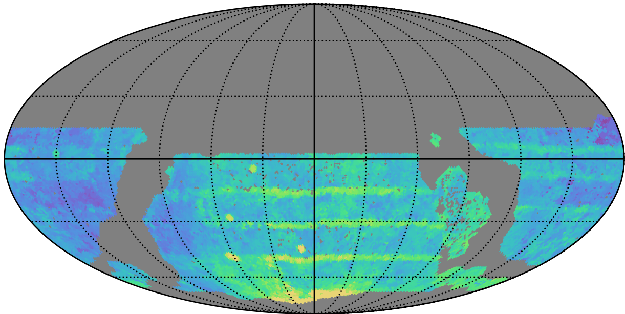
ddf_acor_sf10_lsf30_lsr20_v3.4_10yrs WFD all bands: Median Season Length
