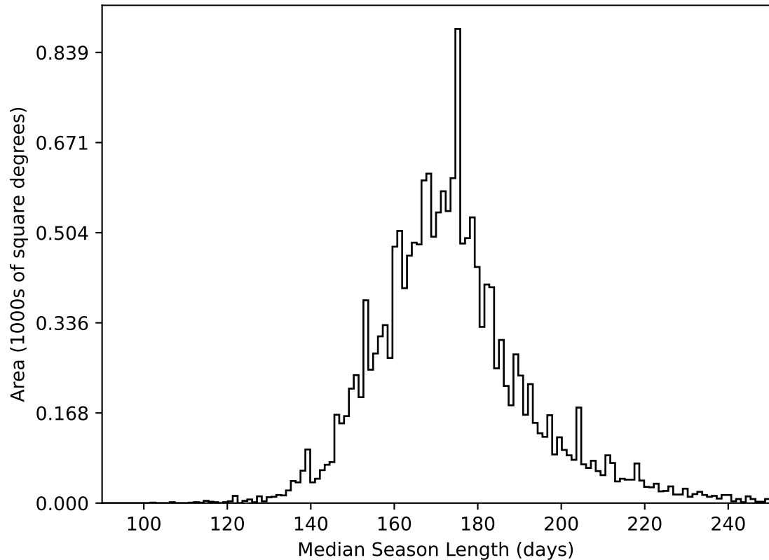
ddf_acor_sf10_lsf30_lsr20_v3.4_10yrs WFD all bands: Median Season Length
