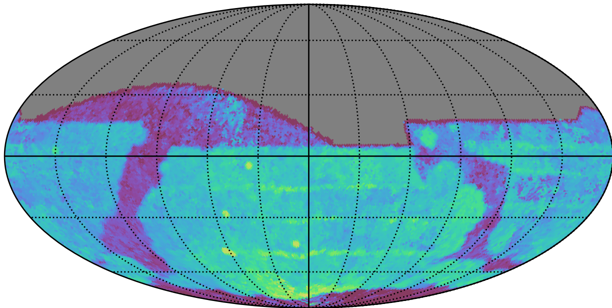
ddf_acor_sf10_lsf30_lsr20_v3.4_10yrs All sky z band: Median Season Length
