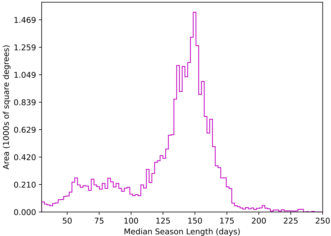
ddf_acor_sf10_lsf30_lsr20_v3.4_10yrs All sky z band: Median Season Length
