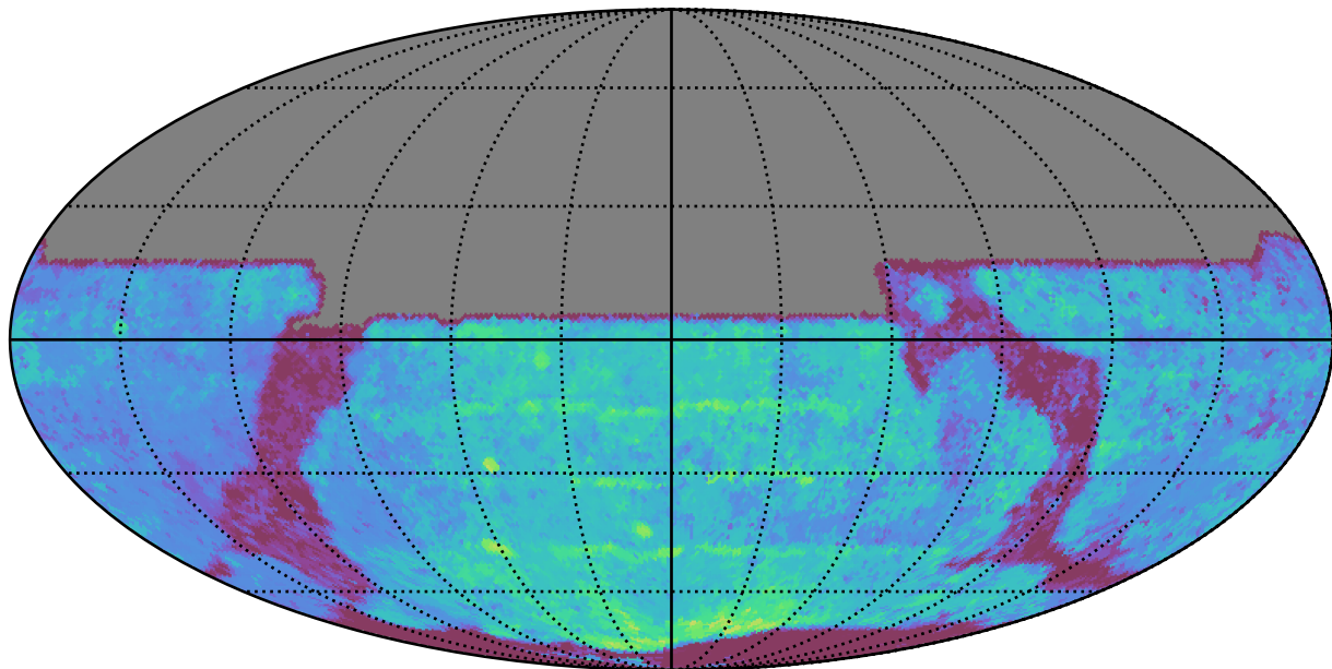
ddf_acor_sf10_lsf30_lsr20_v3.4_10yrs All sky y band: Median Season Length
