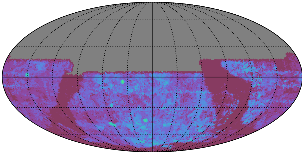
ddf_acor_sf10_lsf30_lsr20_v3.4_10yrs All sky u band: Median Season Length
