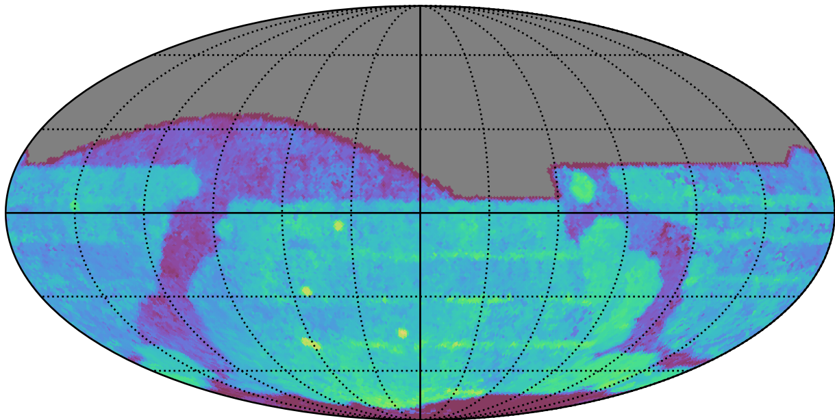
ddf_acor_sf10_lsf30_lsr20_v3.4_10yrs All sky r band: Median Season Length
