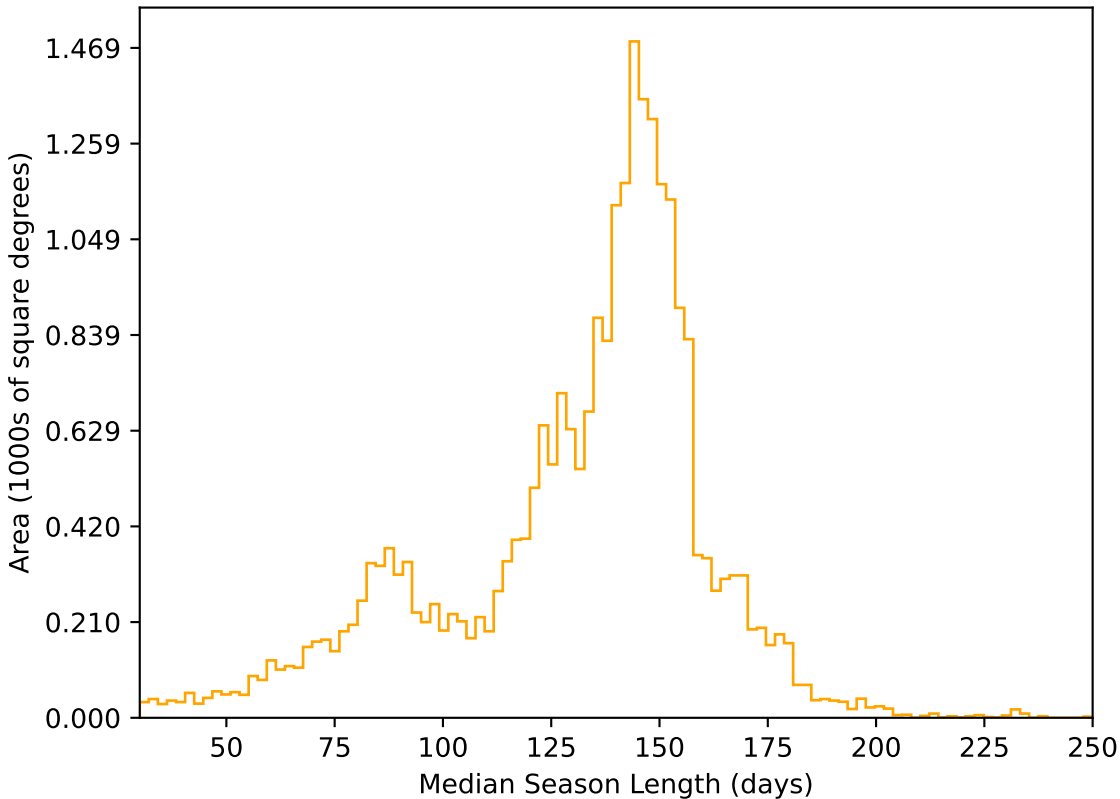
ddf_acor_sf10_lsf30_lsr20_v3.4_10yrs All sky r band: Median Season Length
