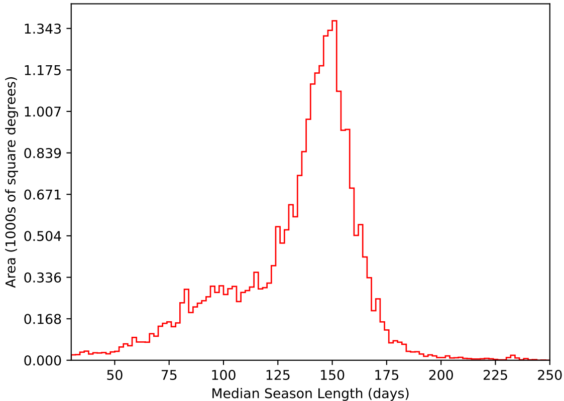
ddf_acor_sf10_lsf30_lsr20_v3.4_10yrs All sky i band: Median Season Length
