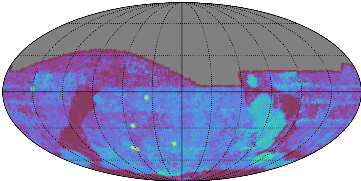
ddf_acor_sf10_lsf30_lsr20_v3.4_10yrs All sky g band: Median Season Length
