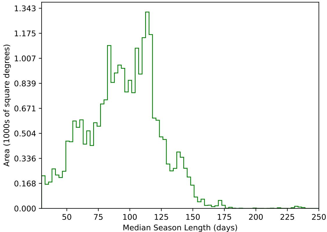
ddf_acor_sf10_lsf30_lsr20_v3.4_10yrs All sky g band: Median Season Length
