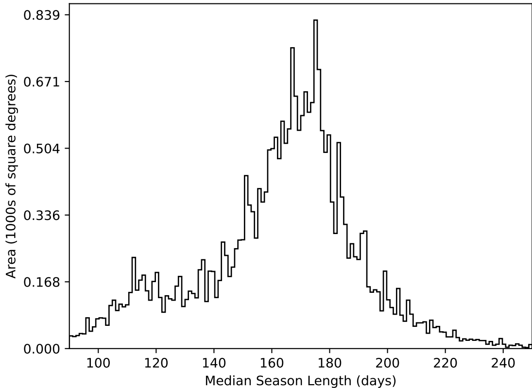
ddf_acor_sf10_lsf30_lsr20_v3.4_10yrs All sky all bands: Median Season Length
