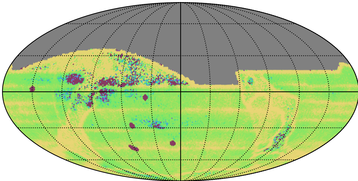
ddf_acor_sf10_lsf30_lsr20_v3.4_10yrs All sky: Median Intra-Night Gap
