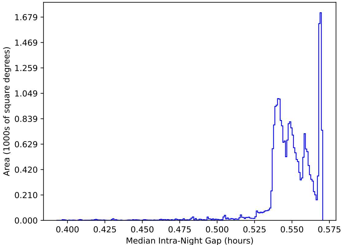
ddf_acor_sf10_lsf30_lsr20_v3.4_10yrs All sky: Median Intra-Night Gap
