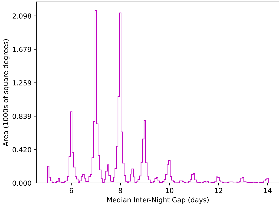
ddf_acor_sf10_lsf30_lsr20_v3.4_10yrs WFD z band: Median Inter-Night Gap
