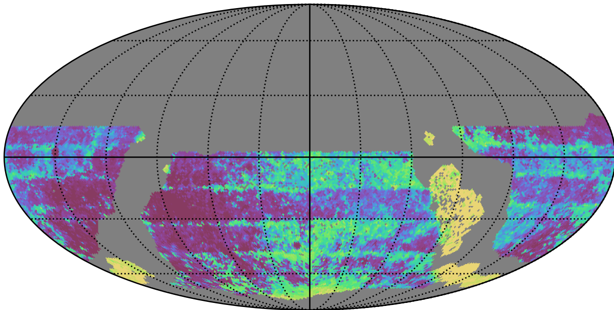
ddf_acor_sf10_lsf30_lsr20_v3.4_10yrs WFD y band: Median Inter-Night Gap
