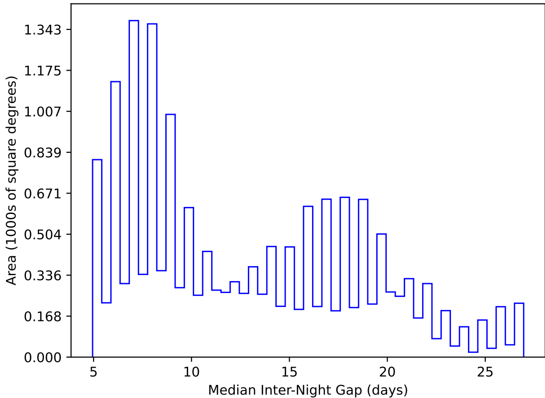
ddf_acor_sf10_lsf30_lsr20_v3.4_10yrs WFD y band: Median Inter-Night Gap
