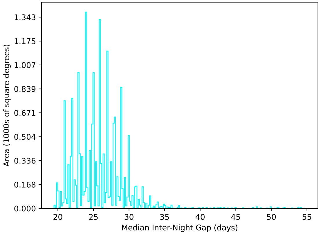
ddf_acor_sf10_lsf30_lsr20_v3.4_10yrs WFD u band: Median Inter-Night Gap
