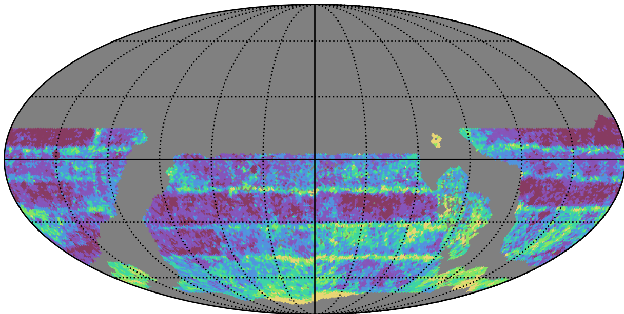
ddf_acor_sf10_lsf30_lsr20_v3.4_10yrs WFD r band: Median Inter-Night Gap
