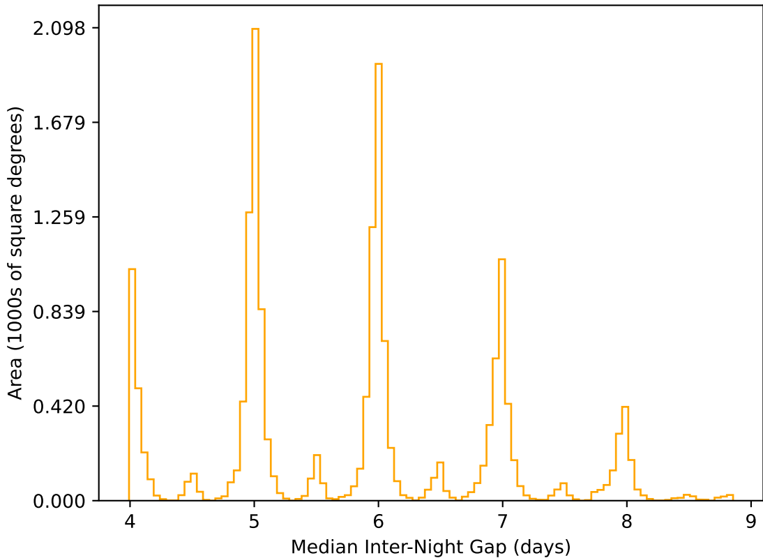
ddf_acor_sf10_lsf30_lsr20_v3.4_10yrs WFD r band: Median Inter-Night Gap
