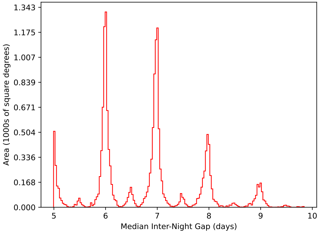
ddf_acor_sf10_lsf30_lsr20_v3.4_10yrs WFD i band: Median Inter-Night Gap
