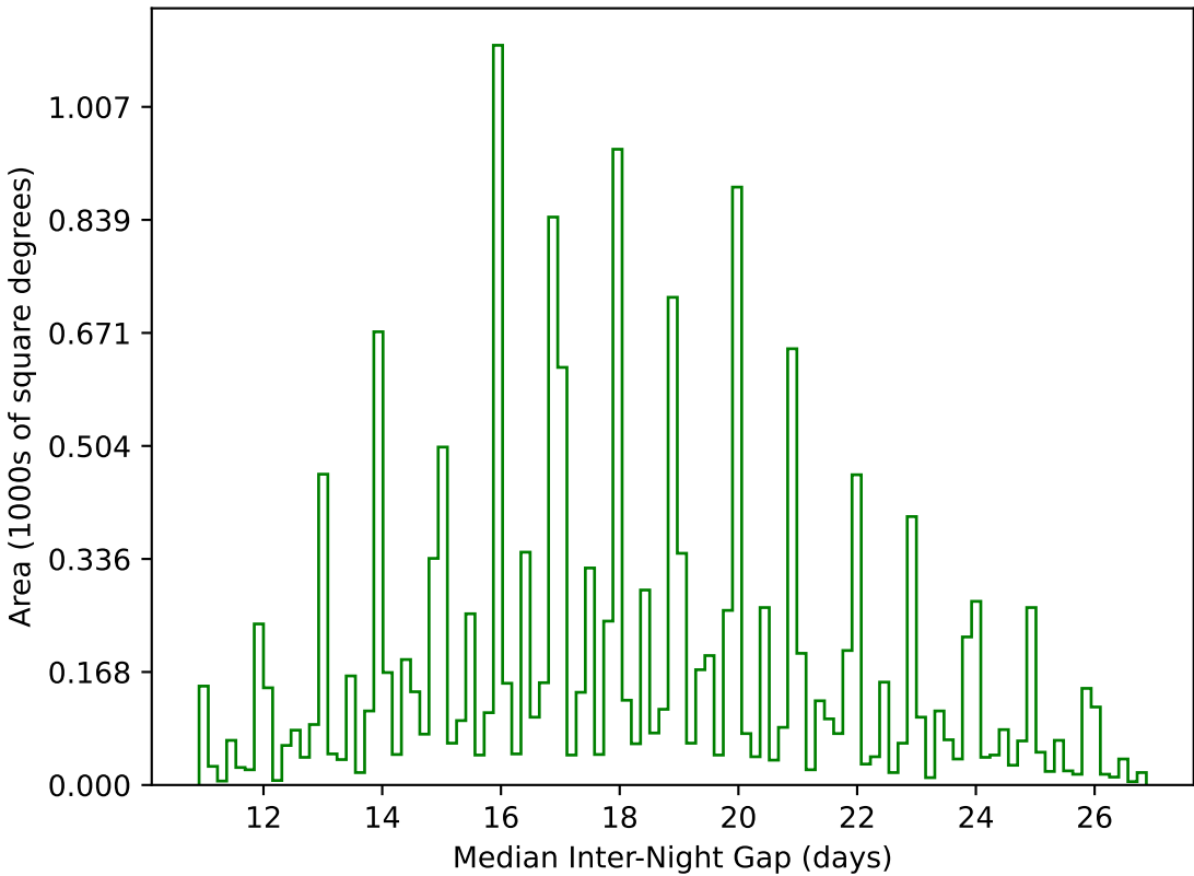
ddf_acor_sf10_lsf30_lsr20_v3.4_10yrs WFD g band: Median Inter-Night Gap
