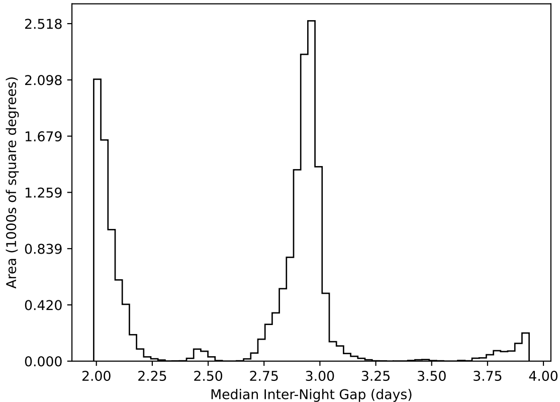
ddf_acor_sf10_lsf30_lsr20_v3.4_10yrs WFD all bands: Median Inter-Night Gap
