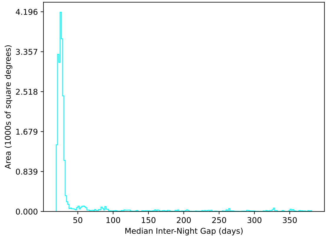
ddf_acor_sf10_lsf30_lsr20_v3.4_10yrs All sky u band: Median Inter-Night Gap
