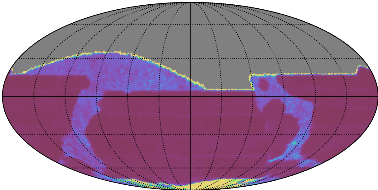
ddf_acor_sf10_lsf30_lsr20_v3.4_10yrs All sky r band: Median Inter-Night Gap
