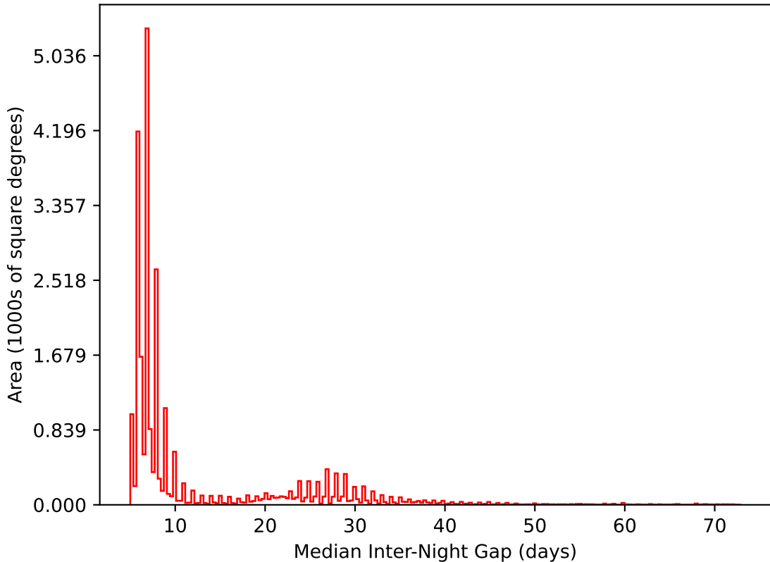
ddf_acor_sf10_lsf30_lsr20_v3.4_10yrs All sky i band: Median Inter-Night Gap
