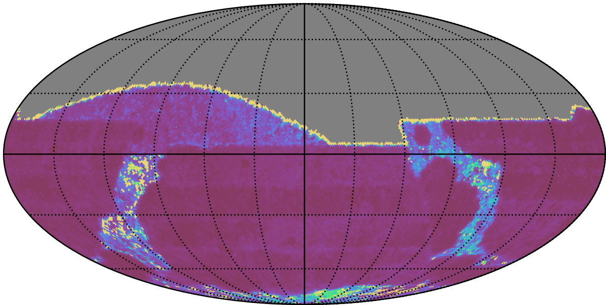
ddf_acor_sf10_lsf30_lsr20_v3.4_10yrs All sky g band: Median Inter-Night Gap
