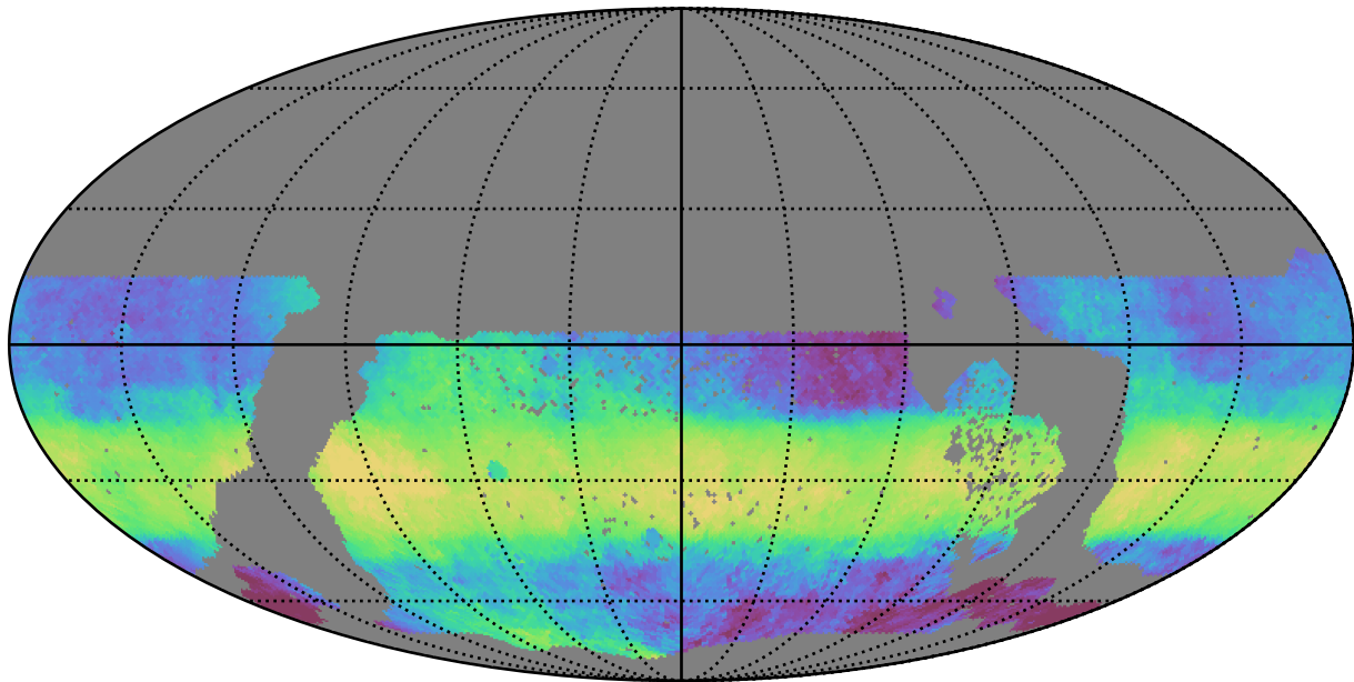
ddf_acor_sf10_lsf30_lsr20_v3.4_10yrs WFD z band: Median HA
