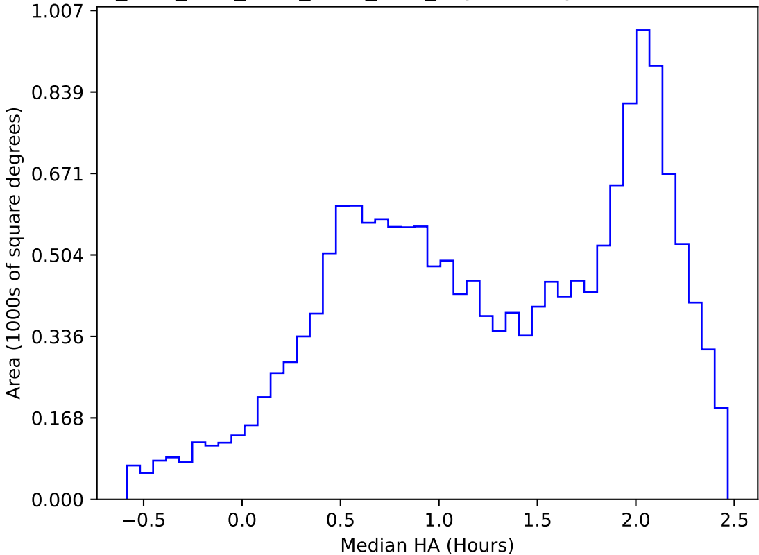
ddf_acor_sf10_lsf30_lsr20_v3.4_10yrs WFD y band: Median HA
