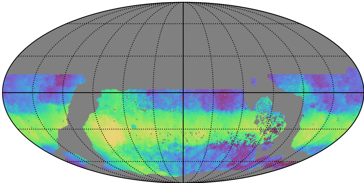
ddf_acor_sf10_lsf30_lsr20_v3.4_10yrs WFD u band: Median HA
