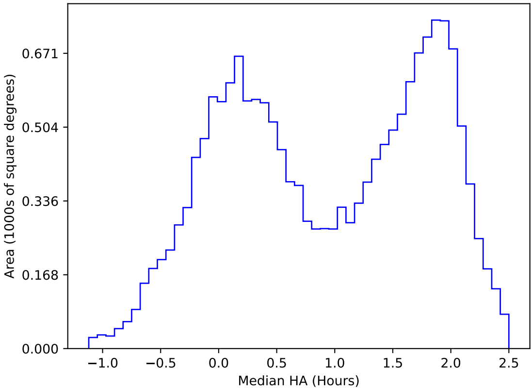
ddf_acor_sf10_lsf30_lsr20_v3.4_10yrs WFD u band: Median HA
