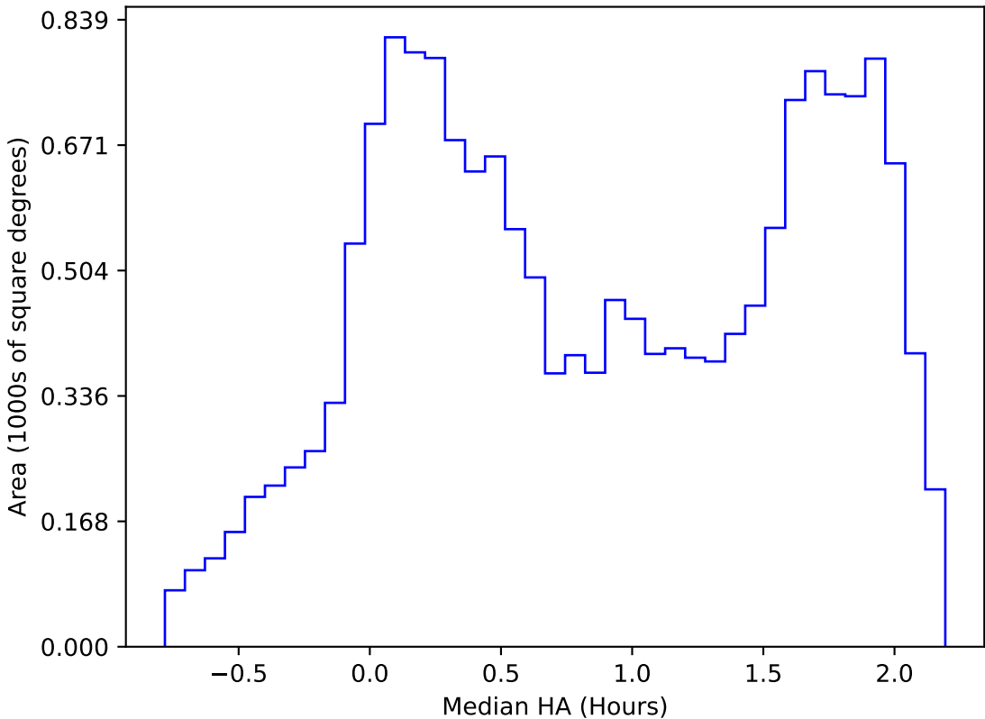
ddf_acor_sf10_lsf30_lsr20_v3.4_10yrs WFD r band: Median HA
