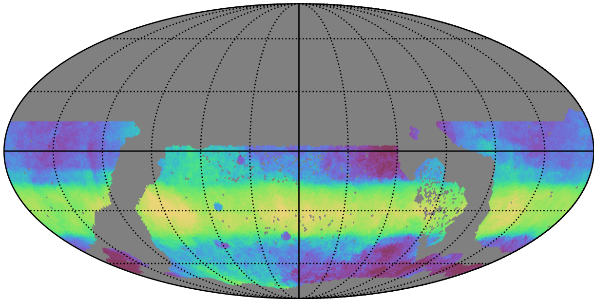
ddf_acor_sf10_lsf30_lsr20_v3.4_10yrs WFD i band: Median HA
