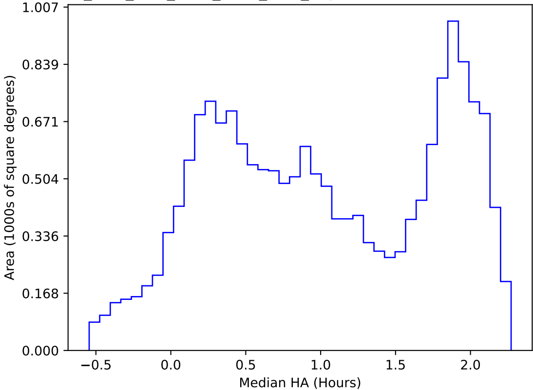
ddf_acor_sf10_lsf30_lsr20_v3.4_10yrs WFD i band: Median HA
