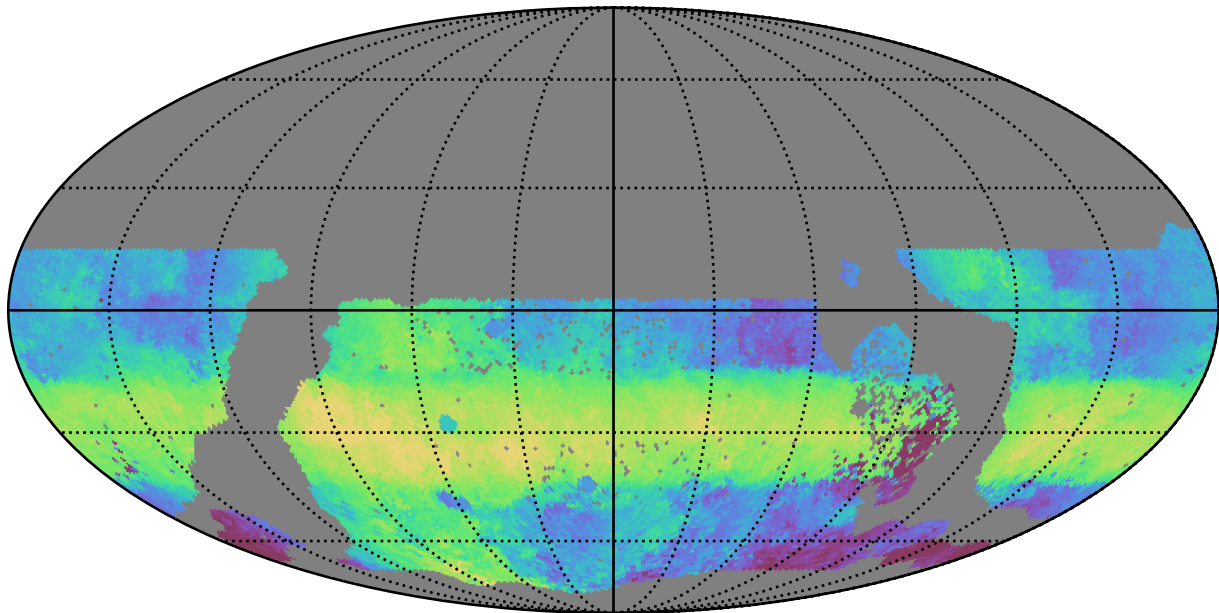
ddf_acor_sf10_lsf30_lsr20_v3.4_10yrs WFD g band: Median HA
