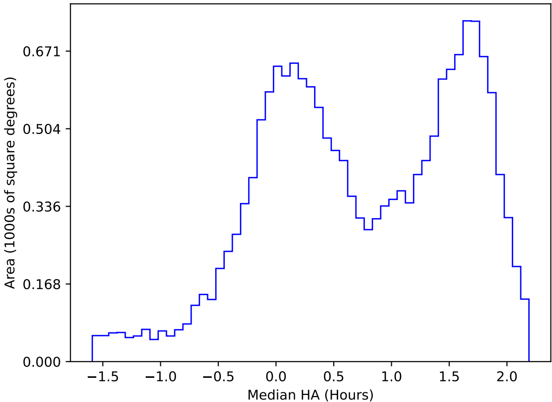
ddf_acor_sf10_lsf30_lsr20_v3.4_10yrs WFD g band: Median HA
