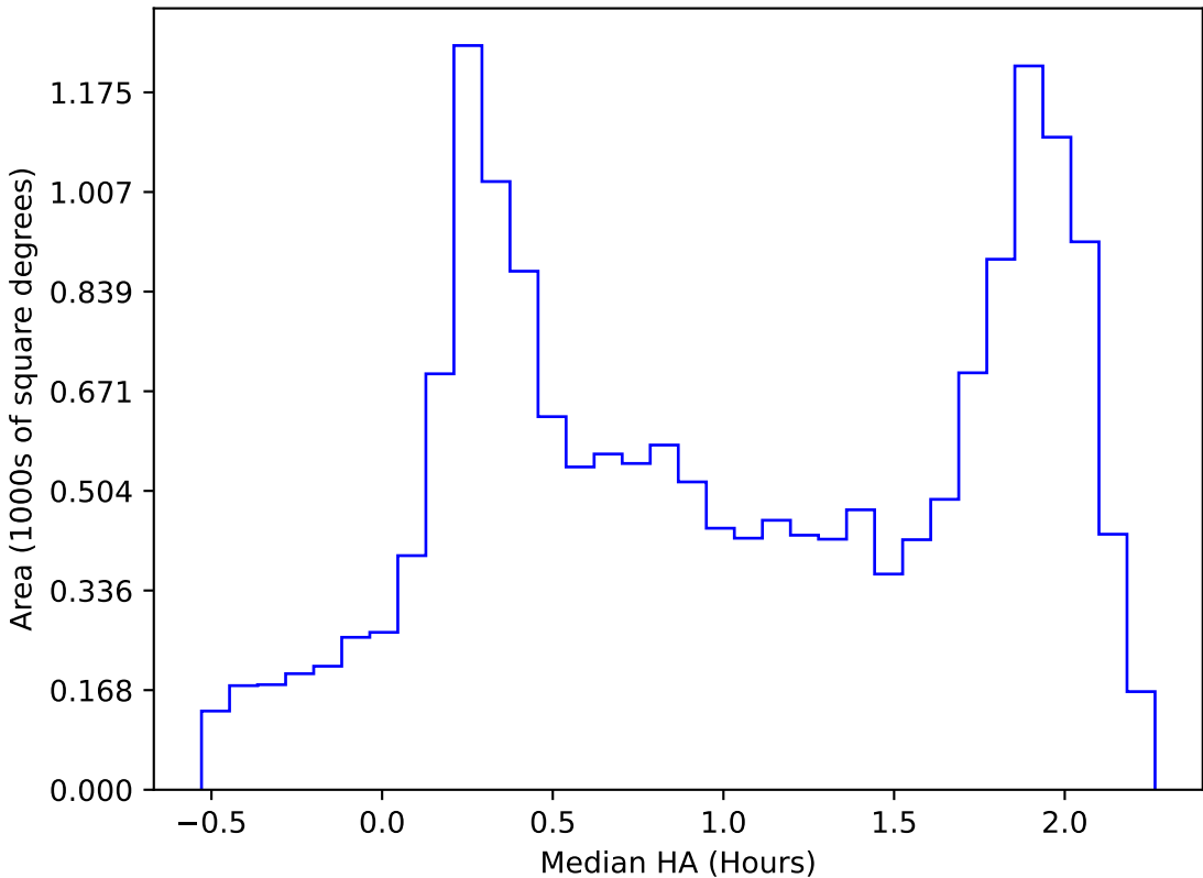
ddf_acor_sf10_lsf30_lsr20_v3.4_10yrs WFD all bands: Median HA
