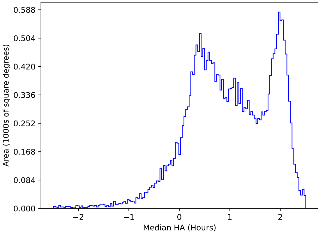
ddf_acor_sf10_lsf30_lsr20_v3.4_10yrs All sky z band: Median HA
