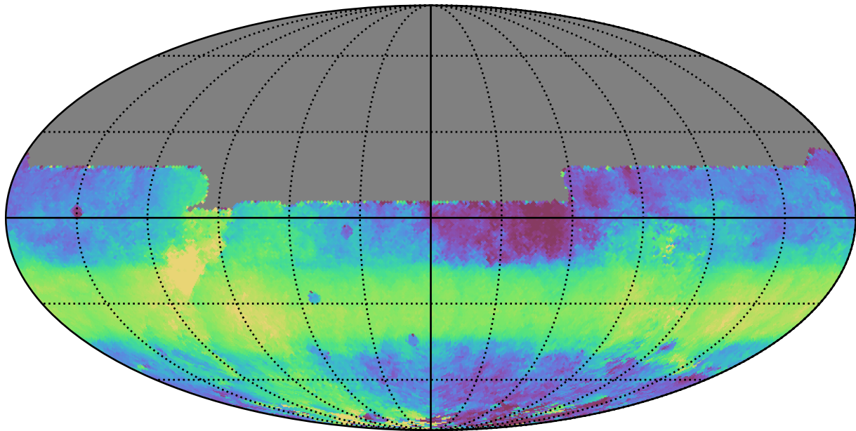
ddf_acor_sf10_lsf30_lsr20_v3.4_10yrs All sky y band: Median HA
