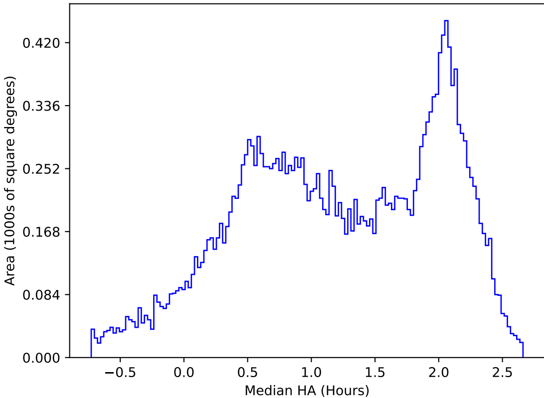
ddf_acor_sf10_ls30_lsr20_v3.4_10yrs All sky y band: Median HA
