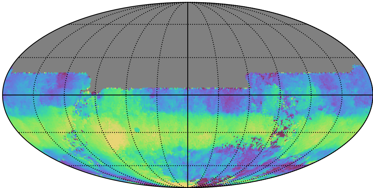
ddf_acor_sf10_lsf30_lsr20_v3.4_10yrs All sky u band: Median HA
