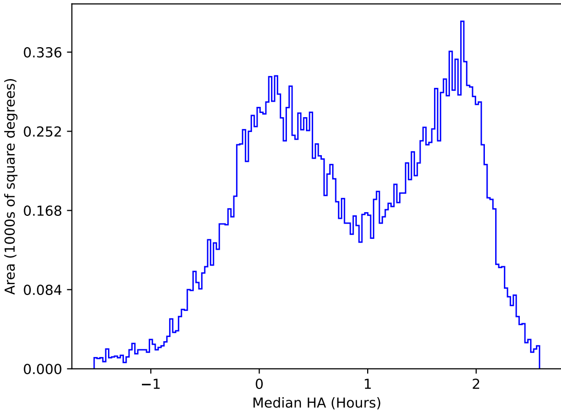
ddf_acor_sf10_ls30_lsr20_v3.4_10yrs All sky u band: Median HA
