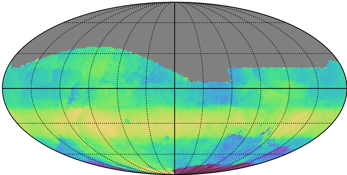
ddf_acor_sf10_lsf30_lsr20_v3.4_10yrs All sky r band: Median HA
