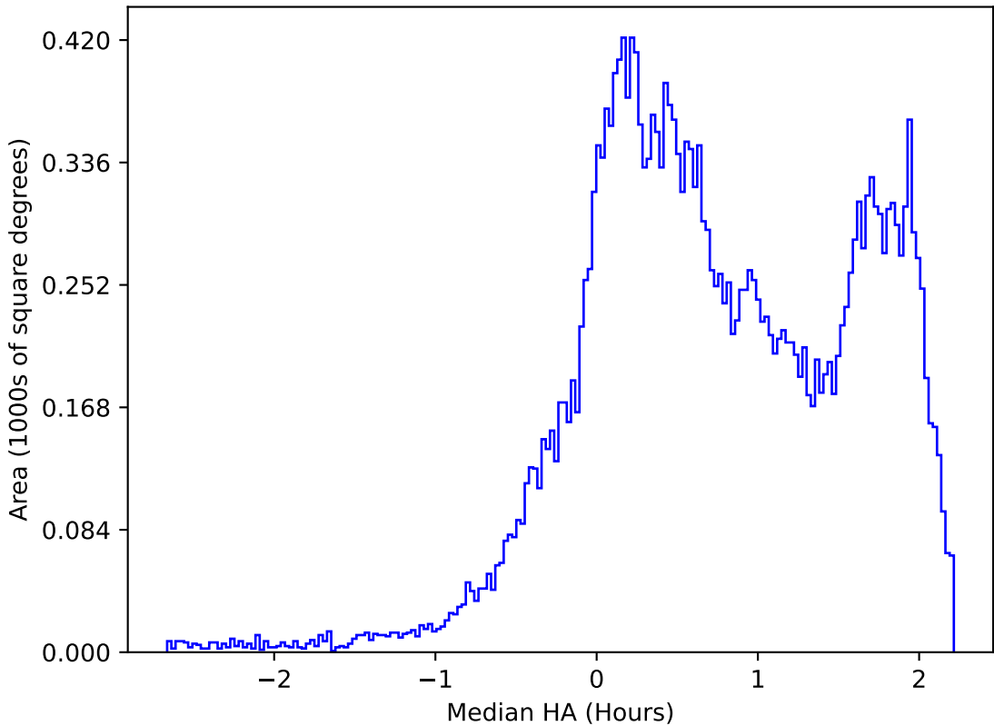
ddf_acor_sf10_lsf30_lsr20_v3.4_10yrs All sky r band: Median HA
